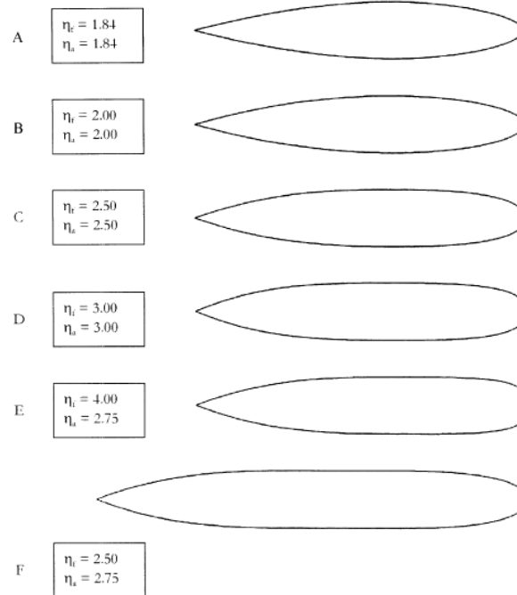
Figure 6: Hull form with coefficients of \eta_a , \eta_f [21]
