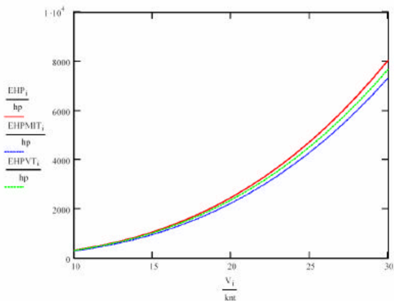
Figure 32 - Plot of EHP vs. speed
