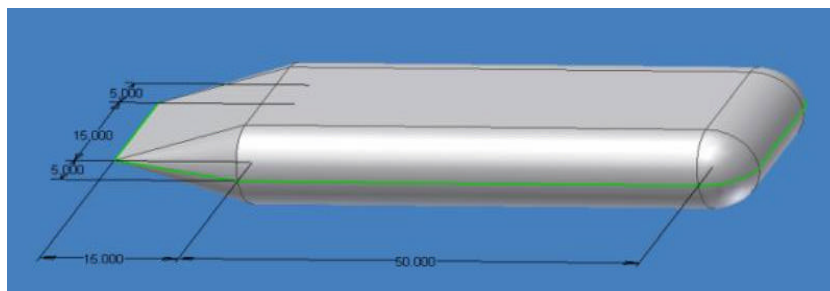
Figure 4 - Idealized Hullform
