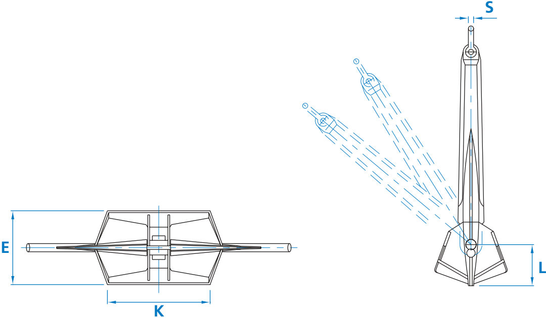
Stevin Mk3
