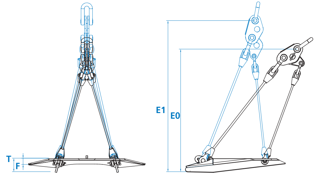
Stevmanta VLA - permanent
