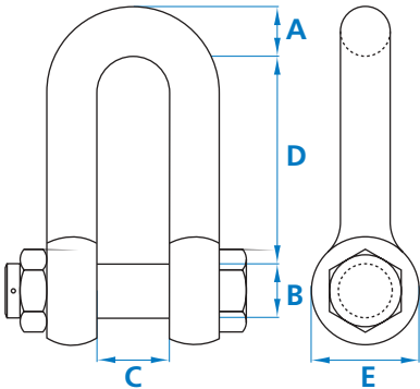
Chain shackle
