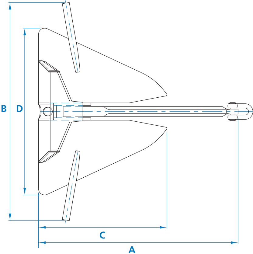
Stevin Mk3
