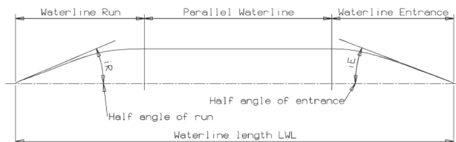
Figure 54: Waterline characteristics
