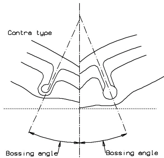
Figure 13: Propeller shaft bossings
