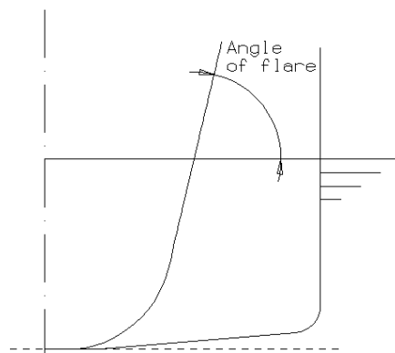
Figure 24: Transverse ship section with flare
