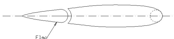
Figure 23: Hydrofoil with flap
