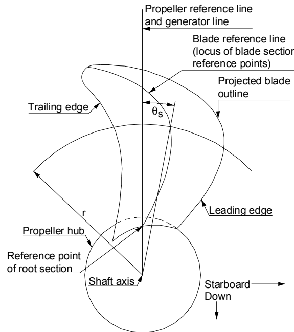
Figure 25: Diagram showing recommended reference lines (looking forward)
