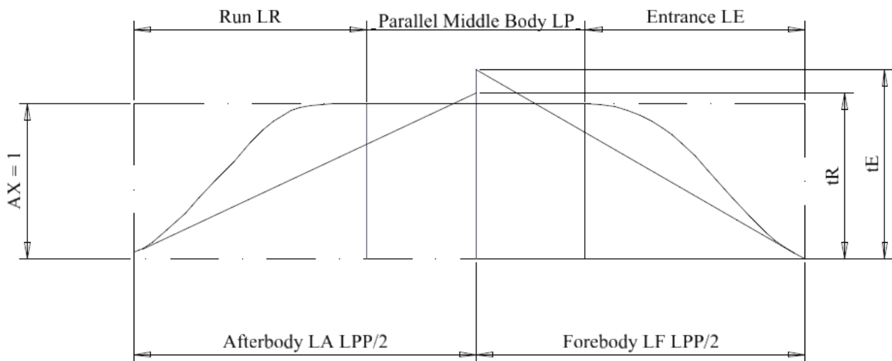
Figure 44: Characteristics of sectional area curve
