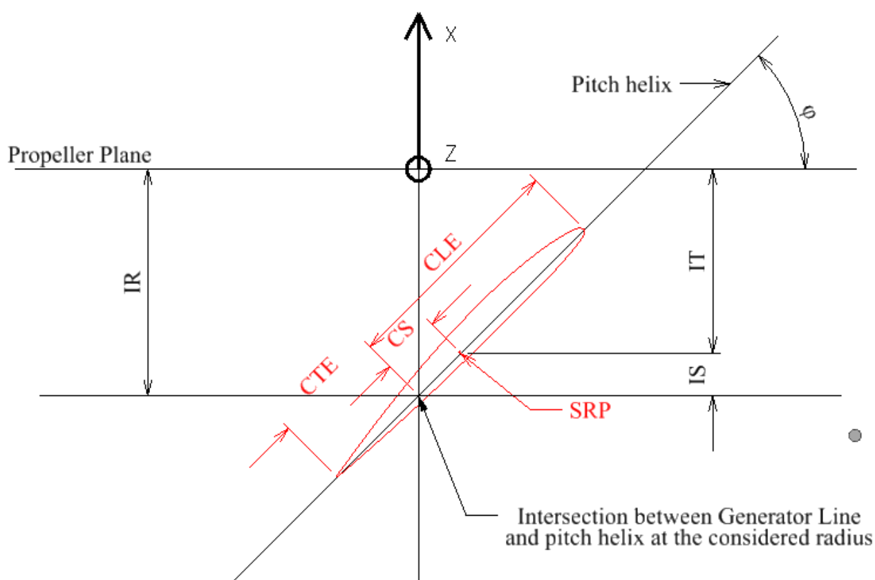
Figure 17: View of unrolled cylindrical section at radius r of a right-handed propeller (looking down) showing subdivisions of the Chord, Skewback and Rake.
