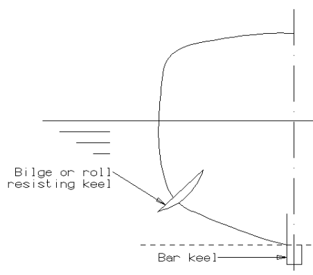
Figure 28: Bilge and bar keels
