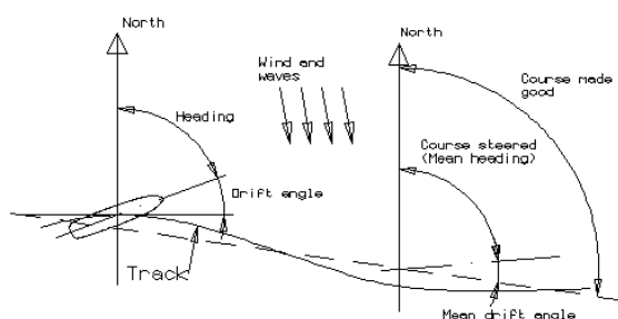
Figure 20: Course characteristics
