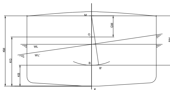
Figure 32: Transverse metacentric parameters
