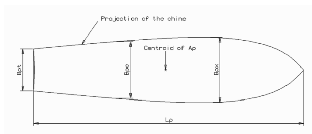
Figure 5: Beam definitions for a hard chine hull
