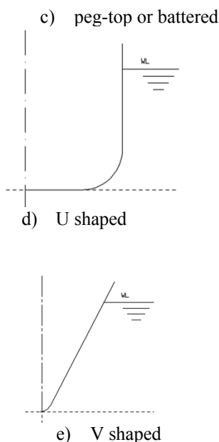
Figure 43: Typical shapes of transverse ship sections
