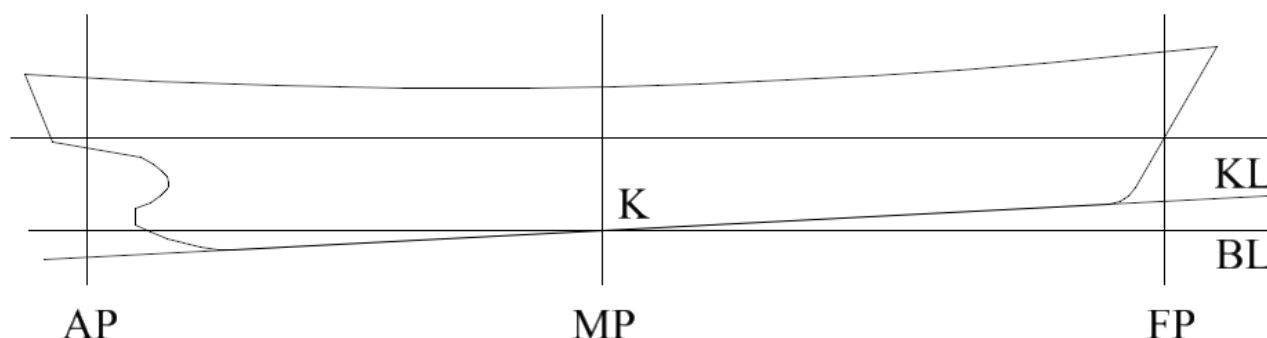
Figure 7: Baseline and Keel Line
