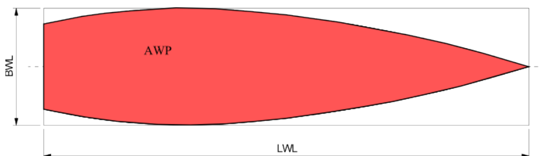
Figure 55: Waterplane area coefficient
