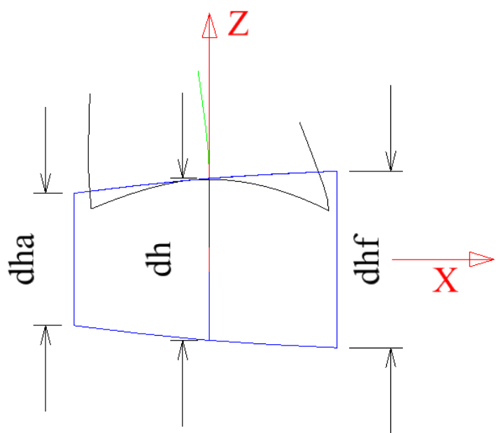
Figure 26: Hub diameters
