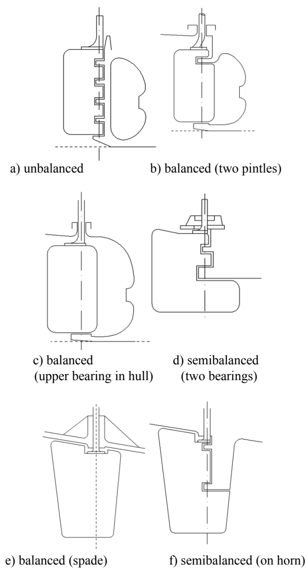
Figure 42: Rudder types
