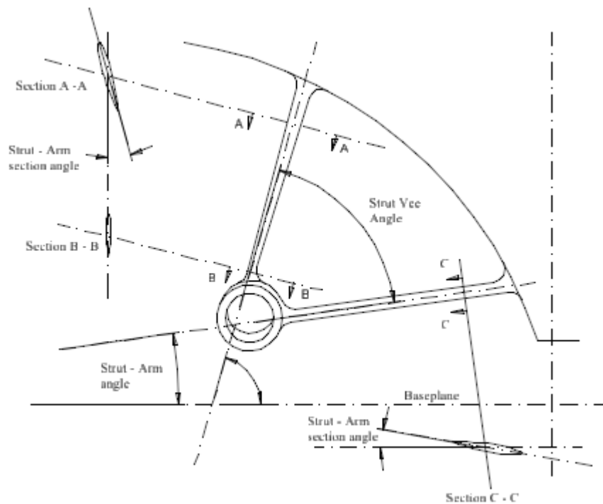
Figure 53: Characteristics of propeller strut or shaft bracket
