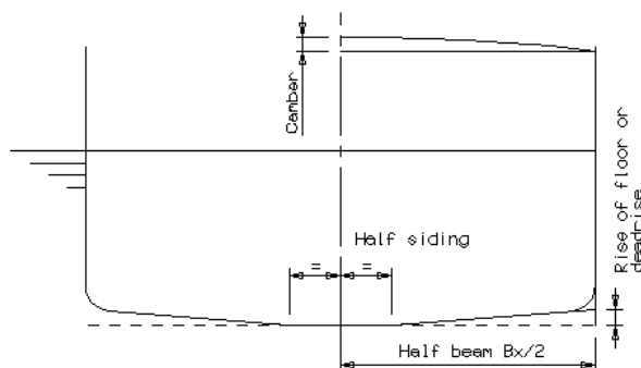
Figure 14: Geometrical characteristics of midship section
