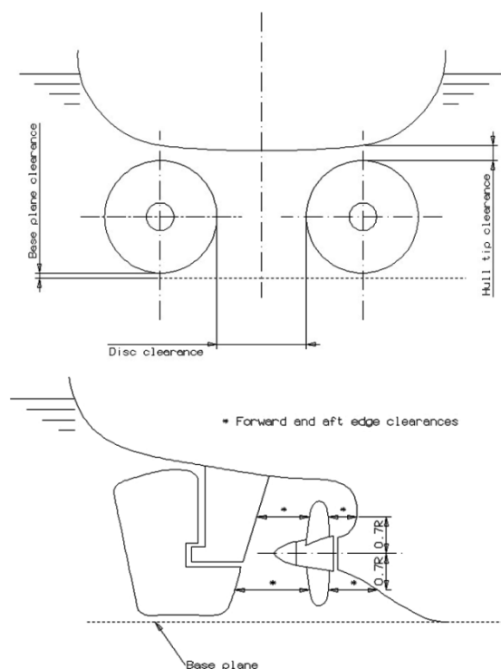
Figure 19: Propeller clearances
