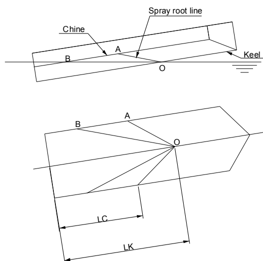
Figure 30: Characteristic ship lengths
