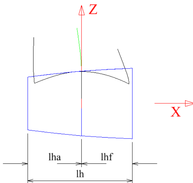
Figure 27: Hub length
