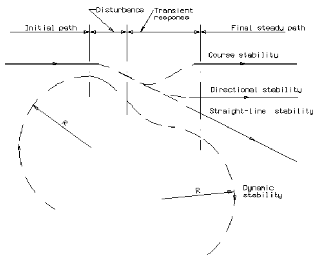
Figure 49: Illustration of stability items
