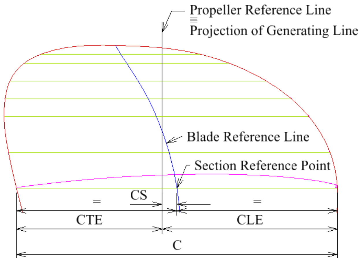
Figure 18: Portion of an expanded blade of a right handed propeller, showing Chord subdivision.
