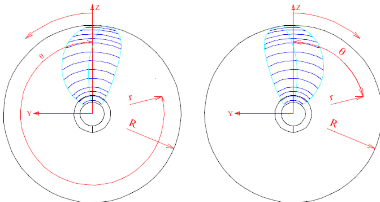
Figure 38: Propeller reference system, cylindrical, looking forward
