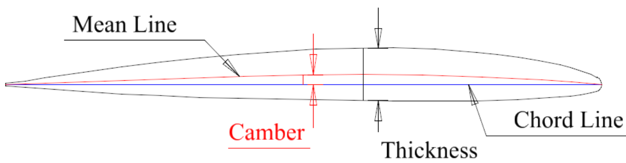
Figure 15: Blade section characteristics
