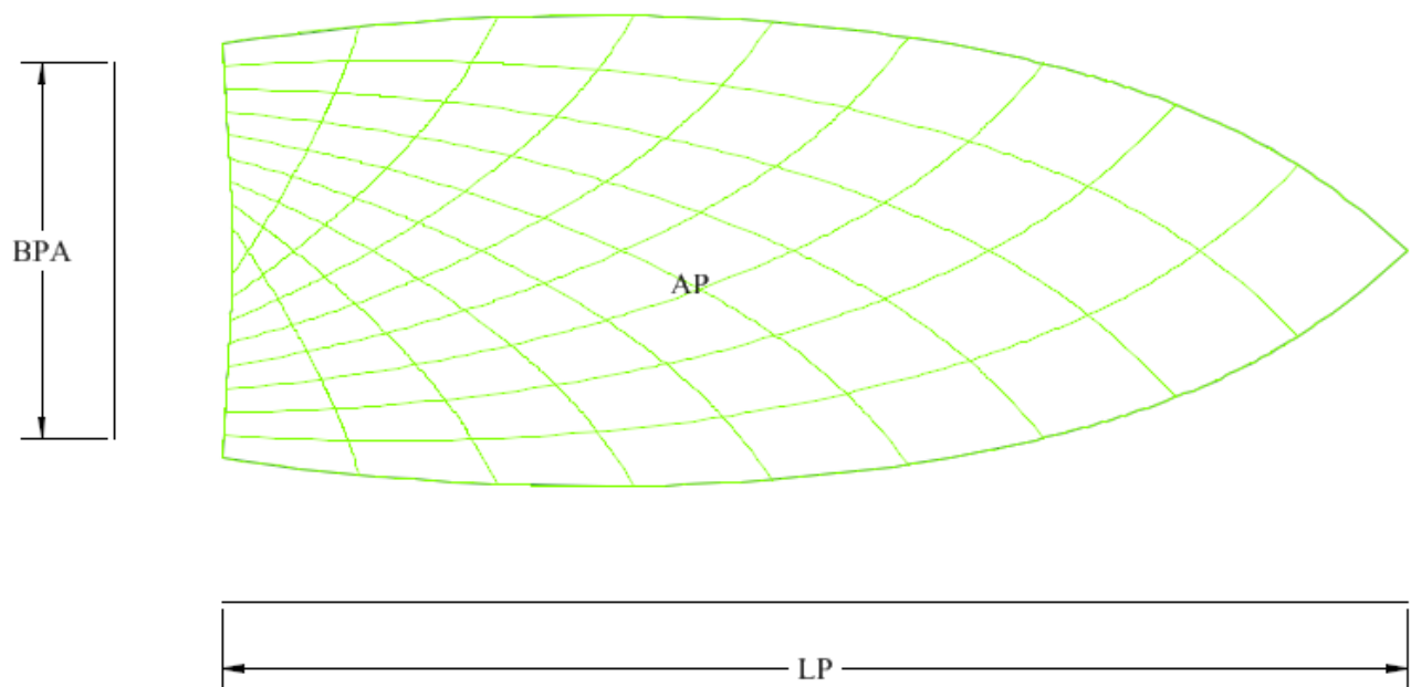
Figure 8: Mean beam over chines
