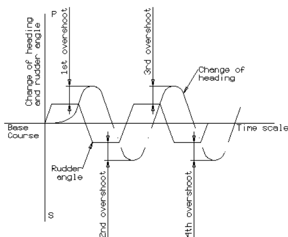
Figure 56: Zigzagging
