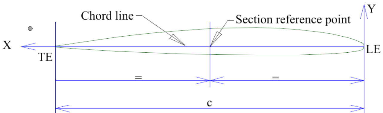
Figure 12: unrolled generic propeller blade section
