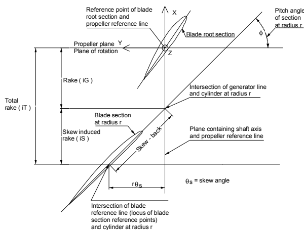
Figure 40: View of unrolled cylindrical sections at blade root and at any radius r of a right-handed propeller (looking down) showing recommended position of propeller plane.
