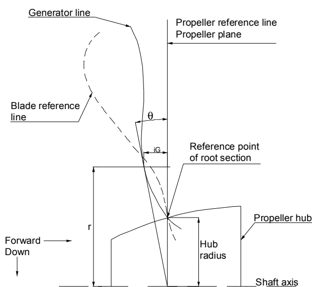
Figure 36: Diagram showing recommended reference lines (looking to port)
