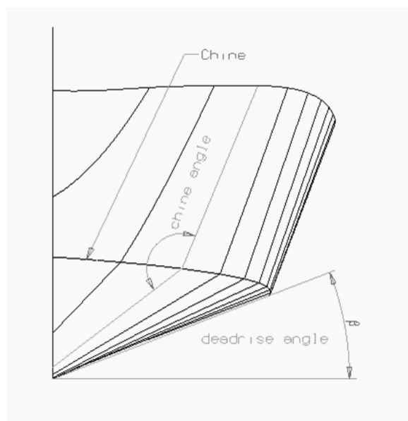
Figure 16: Hull form with chine
