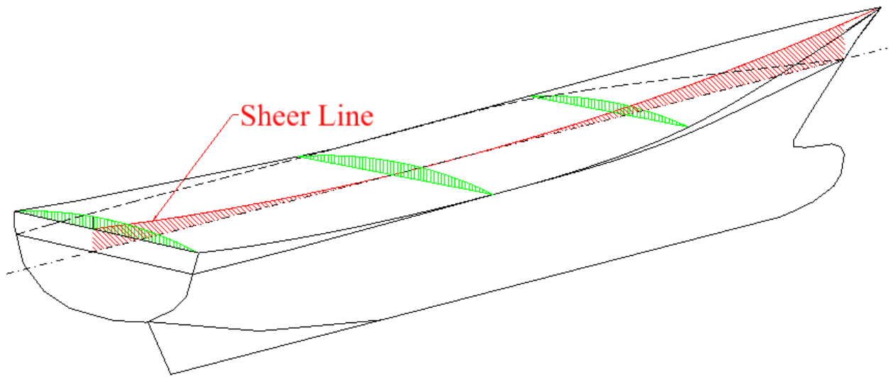
Figure 45: Definition of Sheer line
