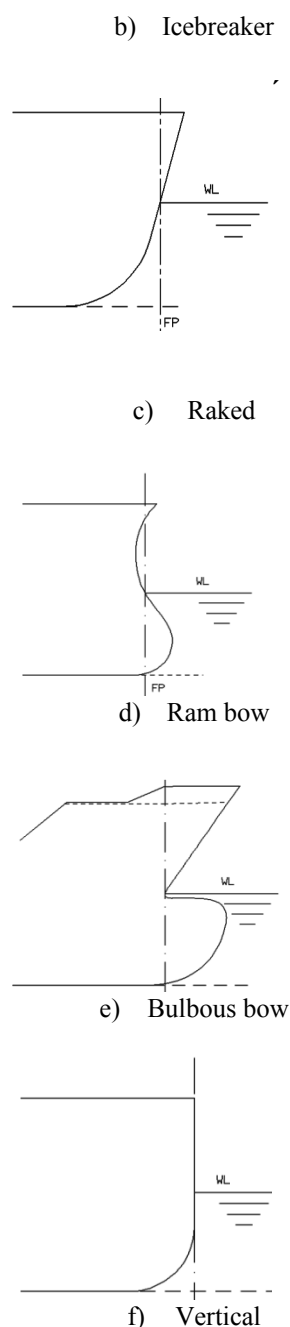
Figure 50: Types of stem profile
