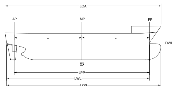
Figure 30: Characteristic ship lengths
