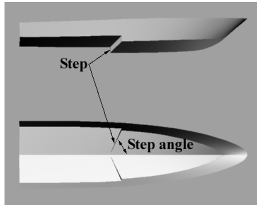
Figure 51: Step in planing craft hull
