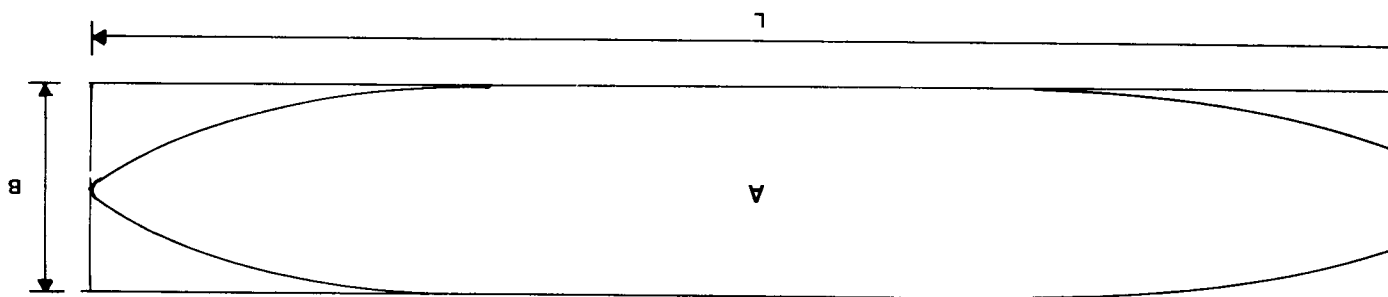
Figure 2.4 (c) Coefficient of fineness of waterplan C_W
