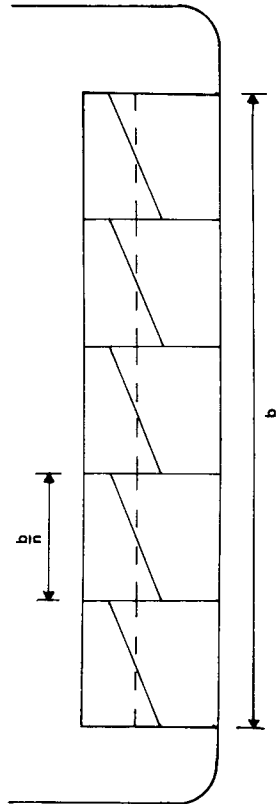
Figure 5.5 Effect of longitudinal subdivision
