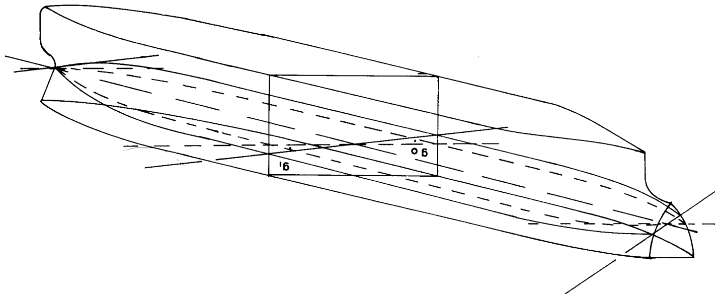
Figure 4.11 Transverse metacentre of a ship shape
