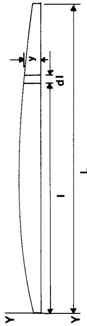
Figure 1.18 Area, second moment and second moment about YY
