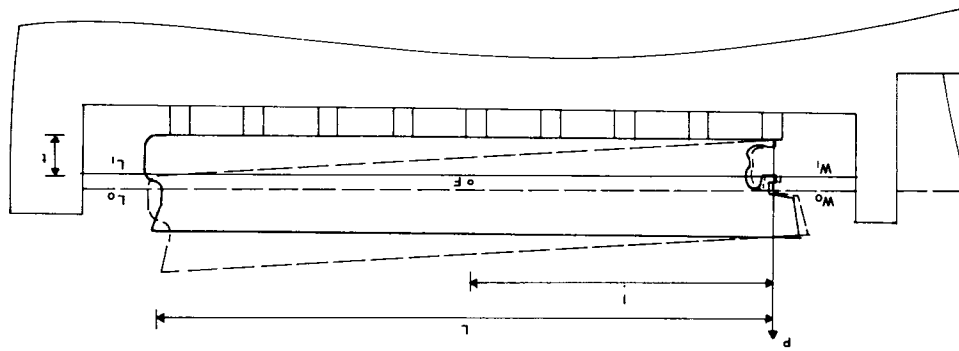
Figure 9.5 Assessment of P at critical instant
