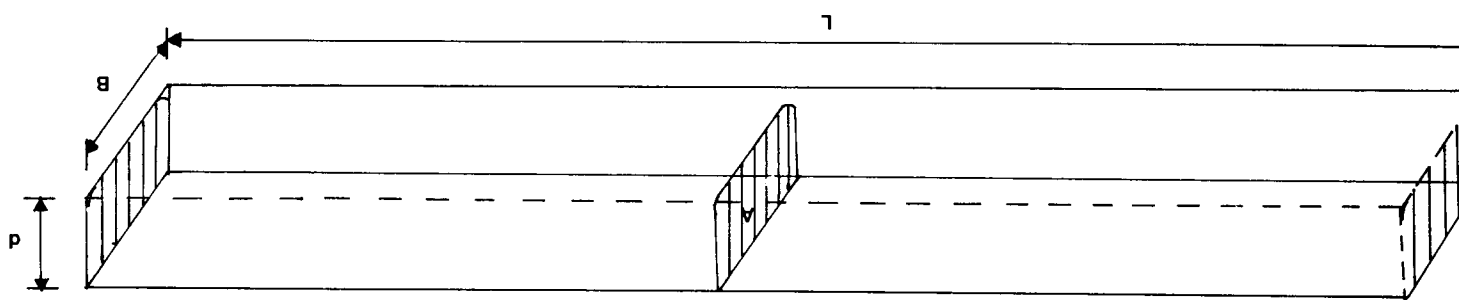
Figure 2.4 (b) Prismatic coefficient
