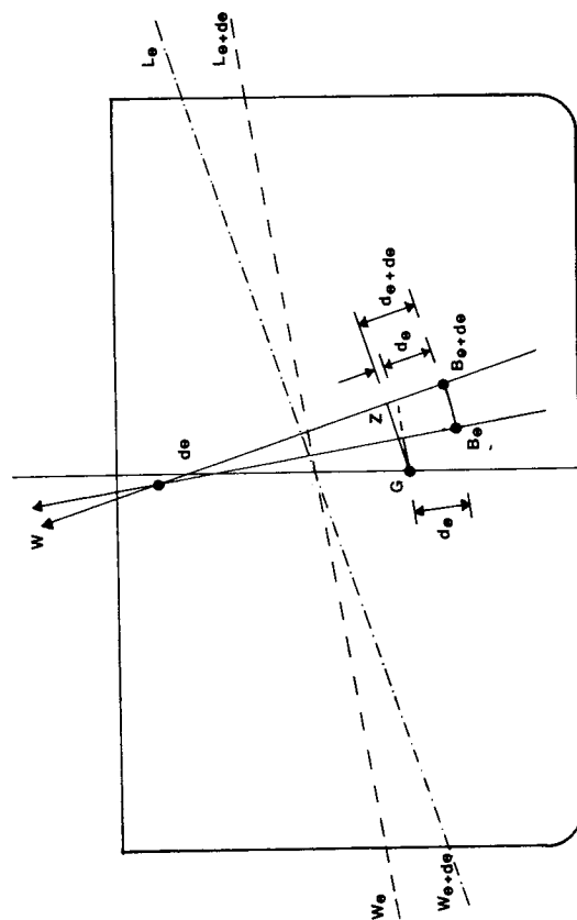
Figure 6.8(a) Relationship between dynamical stability and GZ
