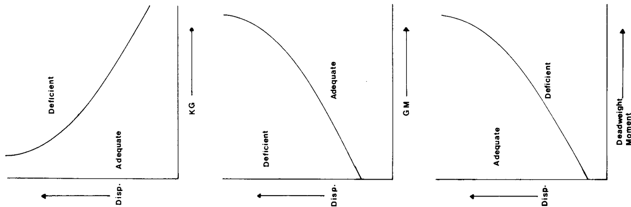
Figure 7.9 Methods of presenting simplified stability data
