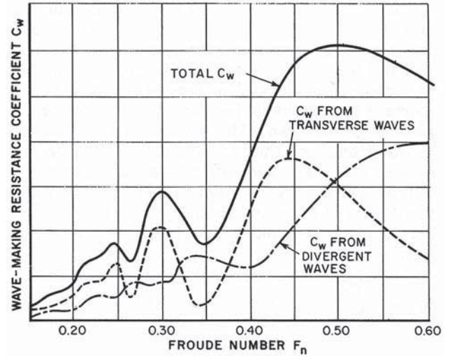
Figure 5.19 Contributions of transverse and divergent waves to wave resistance.
