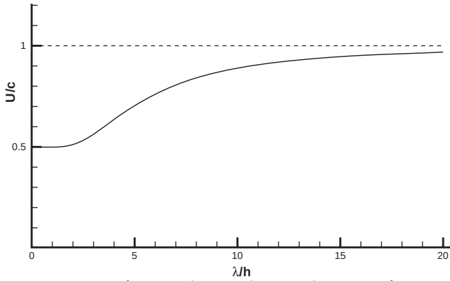
Figure 5.25 Ratio of group velocity and wave velocity, as a function of wave length/water depth ratio.
