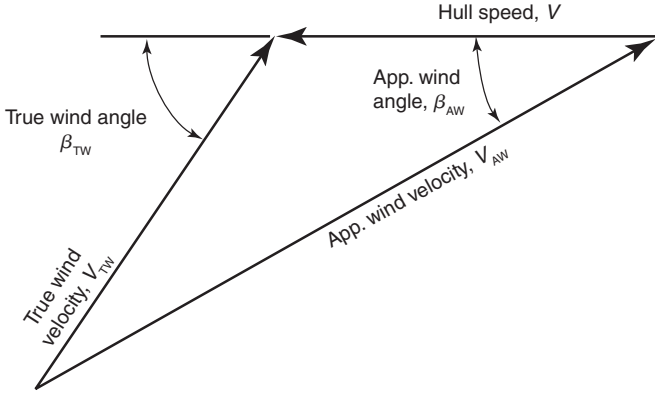
Figure 7.21 Relation between true and apparent wind.
