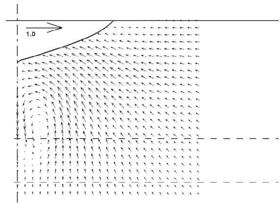
Figure 6.20 Projection of velocity vectors at the propeller plane; model scale.
