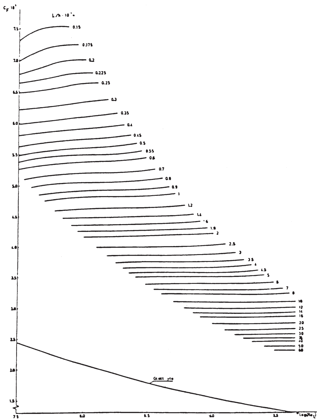
Figure 6.28 Total skin friction coefficient for surfaces covered with densely packed barnacles (Johansson, 1984; courtesy of the Royal Institution of Naval Architects).
