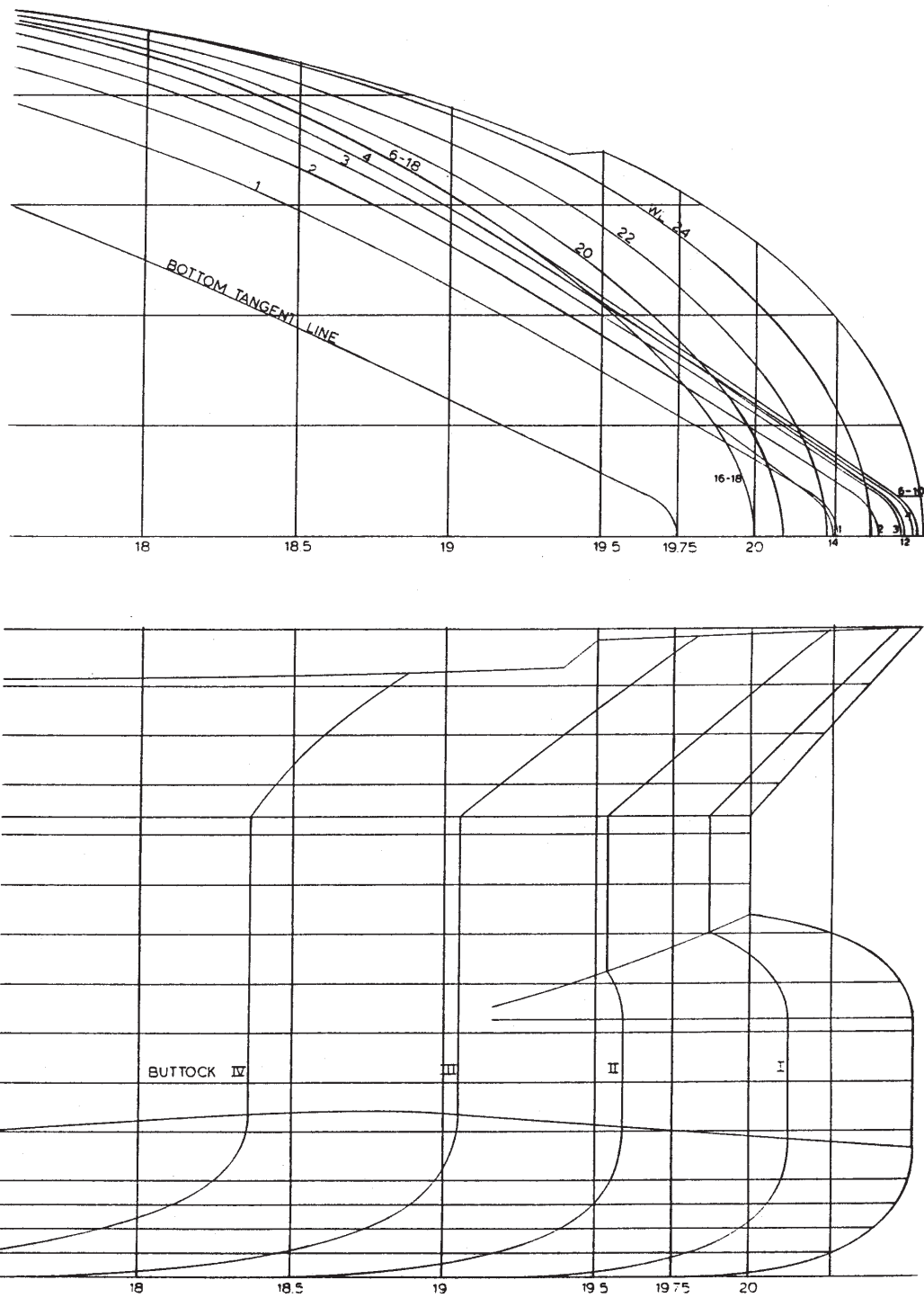
Figure 11.13 A modern bulb for a tanker/bulk carrier (Valkhof, 1999).
