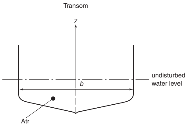
Figure 11.7 Transom definitions.
