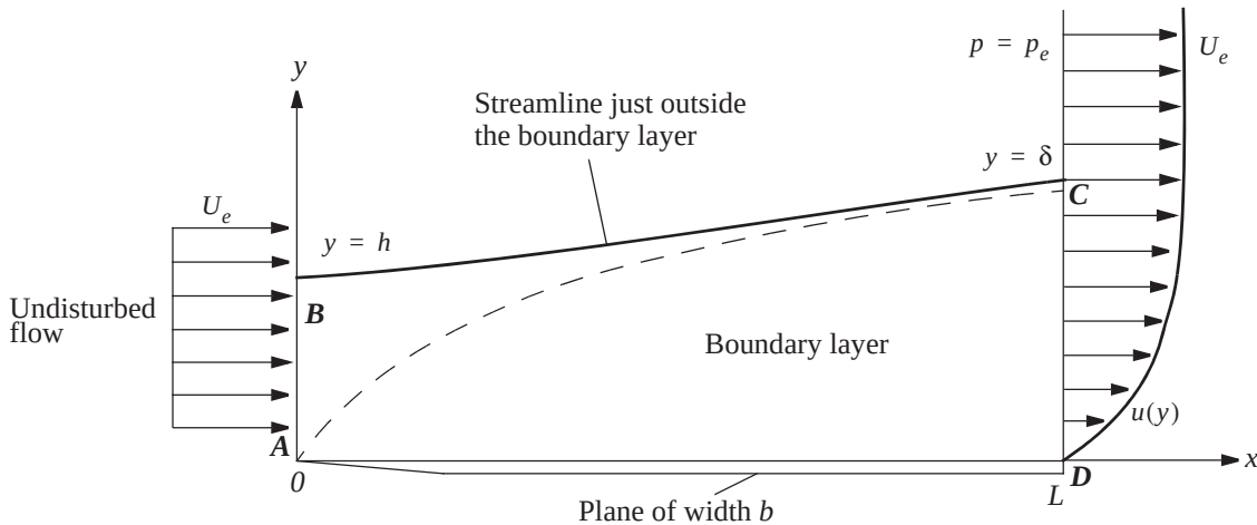
Figure 6.3 Control volume for the derivation of the relation between resistance and momentum thickness.
