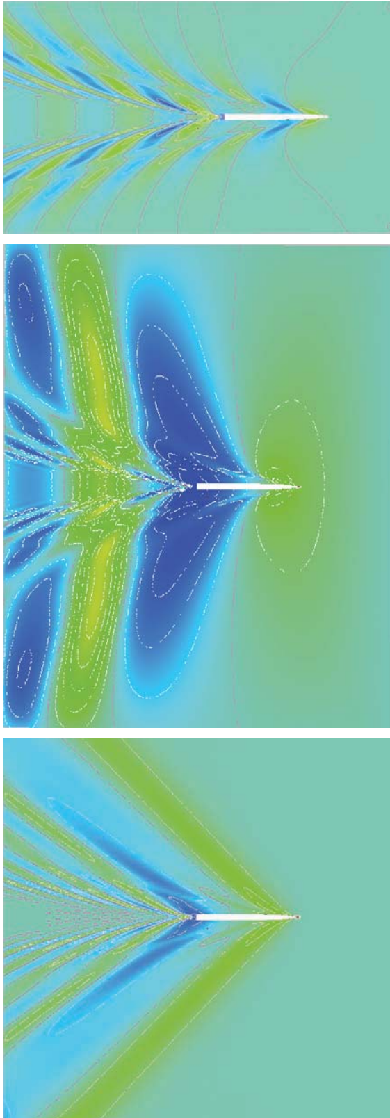
Figure 5.28 Effect of water depth on wave pattern for a ship at Fn_L = 0.35 , as computed. Top to bottom: Fn_h = 0.40 , 0.99 , and 1.40 .
