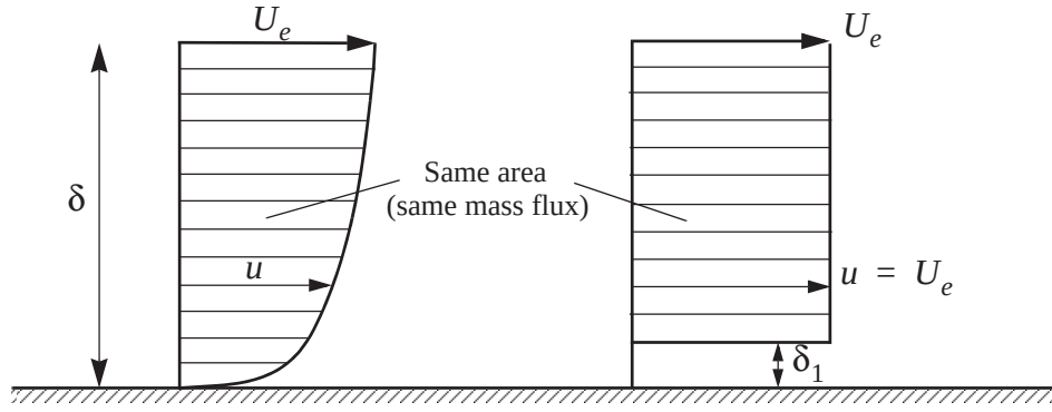
Figure 6.2 Interpretation of the displacement thickness concept.
