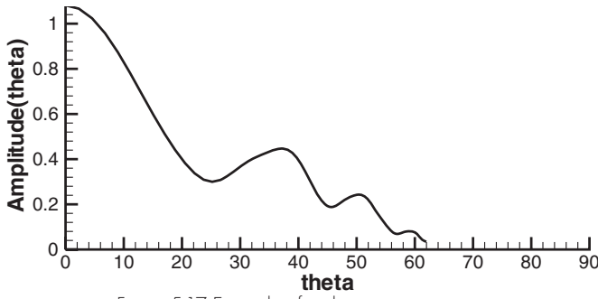
Figure 5.17 Example of a ship wave spectrum.
