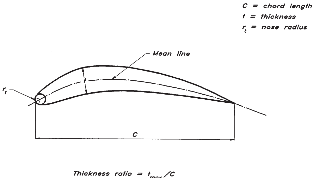
Figure 7.9 Foil section parameters.
