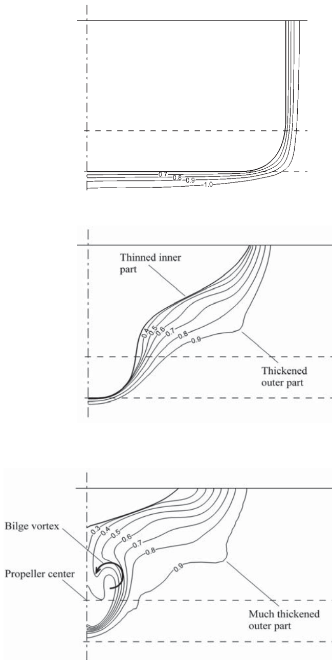
Figure 6.19 Contours of constant axial velocity at three stations, 82.5%, 95.5%, and 99.125% of L_{pp} from the FP. The latter station is the propeller plane. Velocities are nondimensionalized by the undisturbed velocity; model scale.
