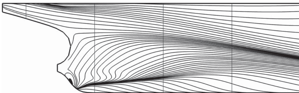
Figure 6.18 Limiting streamlines at the stern, model scale.
