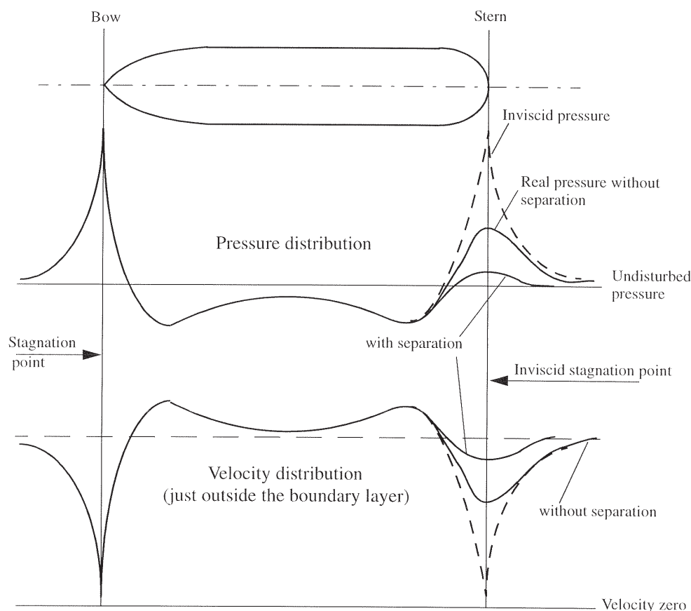
Figure 5.4 Pressure and velocity distribution along a 2D body.
