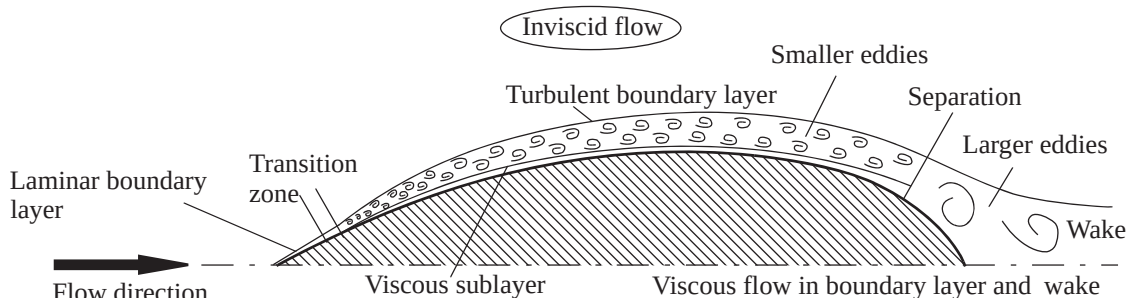
Figure 6.1 Different regions in the flow around the hull.
