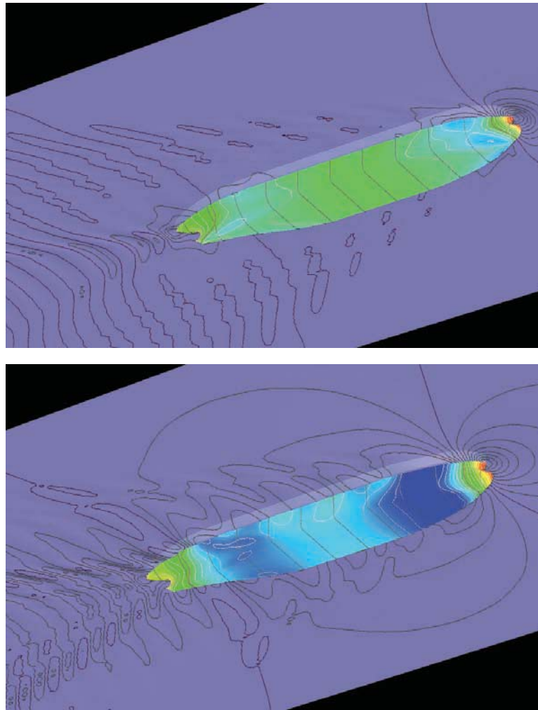
Figure 5.26 Hull pressure distribution and wave pattern for a tanker at F_{n_l} = 0.142 . Top: deep water; bottom: shallow water ( h/T = 1.20 ).
