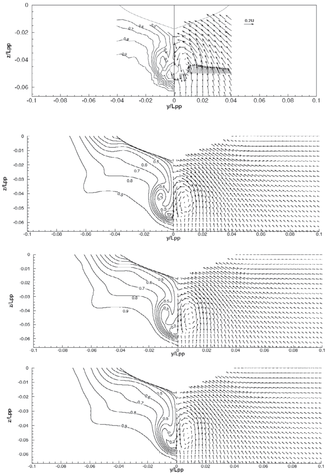
Figure 9.13 Wake contours (left) and cross-flow velocity vectors (right) in the propeller plane of a VLCC (Hino, 2005; courtesy of the author). Top: Experiments; second from top: Reynolds stress model; second from bottom: ASM; bottom: k - \omega SST model.
