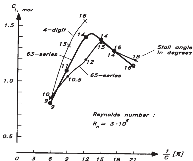
Figure 7.17 Maximum lift coefficient for three sections.
