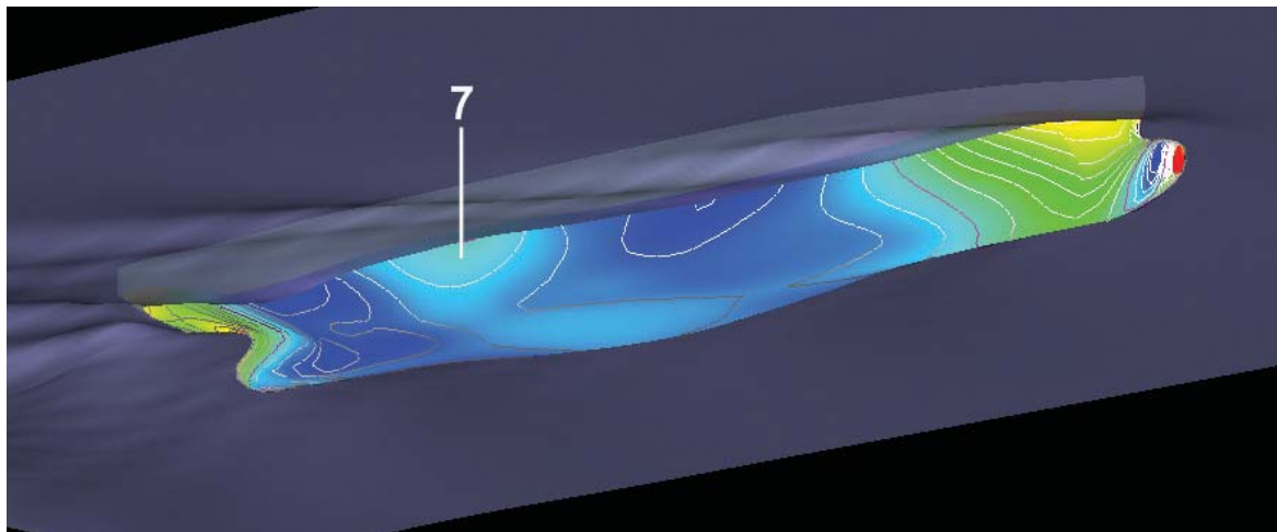
Figure 11.35 Pressure distribution for same hull with free surface, at Fn = 0.28 .
