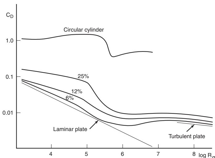
Figure 7.18 Reynolds number dependence of section drag.
