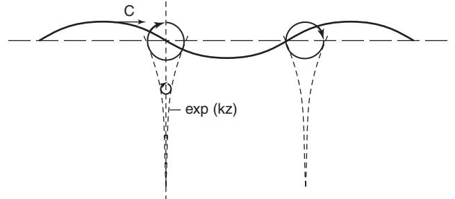
Figure 5.8 Orbital motion in a deep-water wave.
