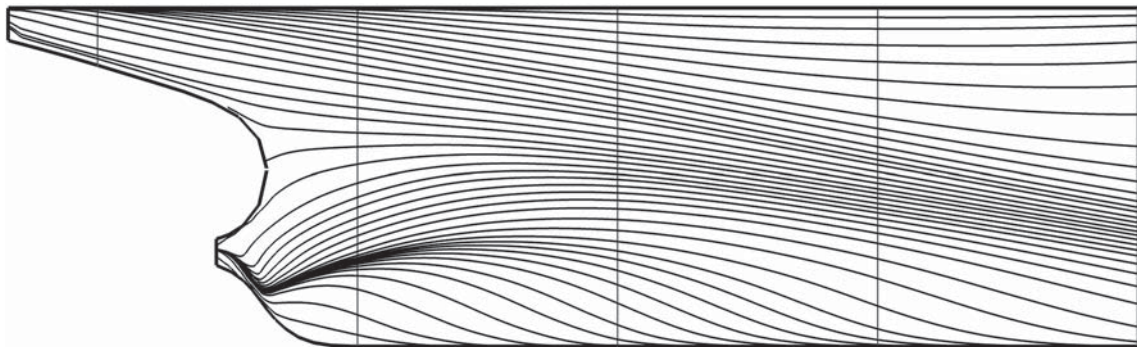
Figure 6.23 Limiting streamlines at full scale.
