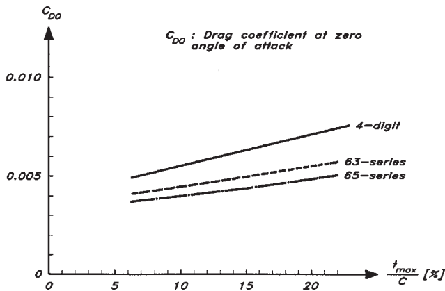
Figure 7.14 Drag at zero angle of attack versus thickness ratio.
