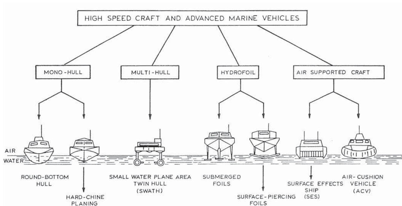
Figure 11.28 Main types of high-speed craft and advanced marine vehicles.
