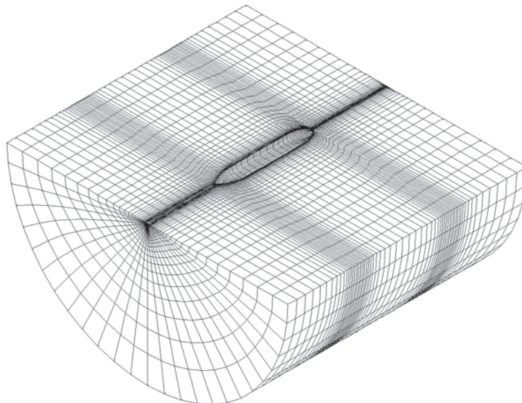
Figure 9.14 Single-block structured grid for a VLCC.
