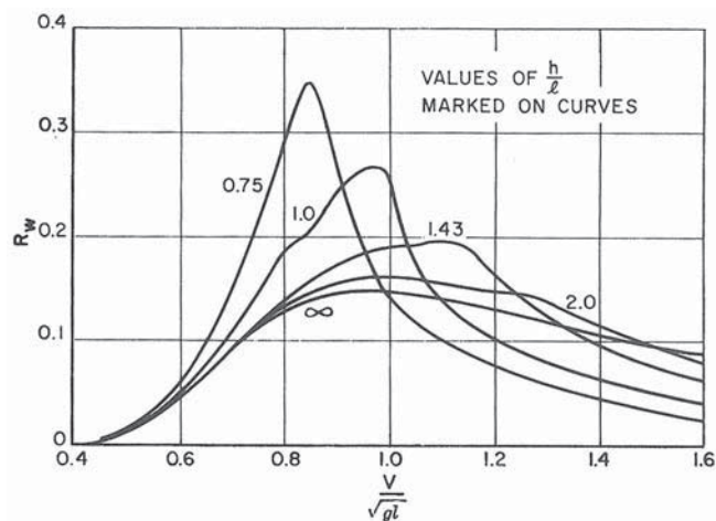
Figure 5.30 Effect of shallow water on wave resistance, according to Havelock (1908).
