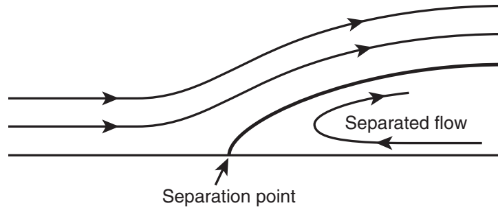
Figure 6.10 Flow near the separation point (S).
