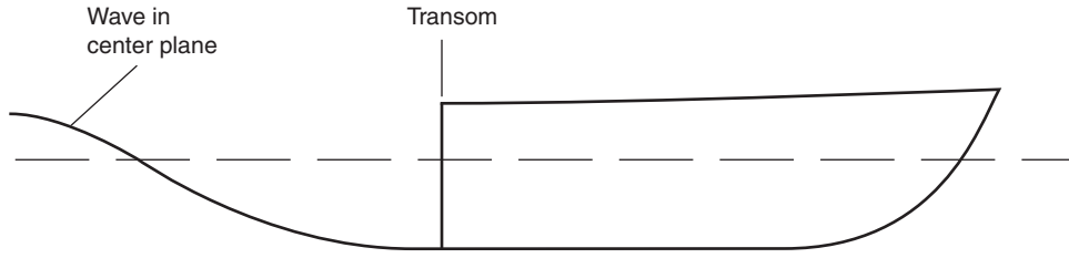
Figure 11.6 Transom stern hull and rooster tail wave (cut through centerplane).
