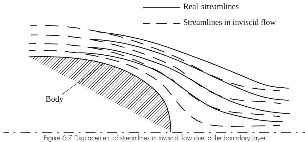
Figure 6.7 Displacement of streamlines in inviscid flow due to the boundary layer.
