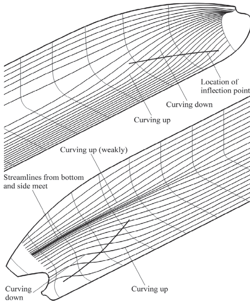
Figure 6.17 Inviscid streamlines on the KVLCC2 hull.
