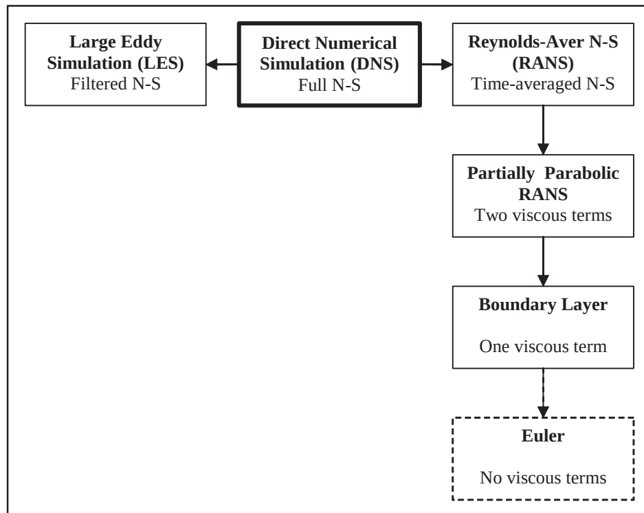
Figure 9.12 Classification of methods used in viscous computational hydrodynamics.
