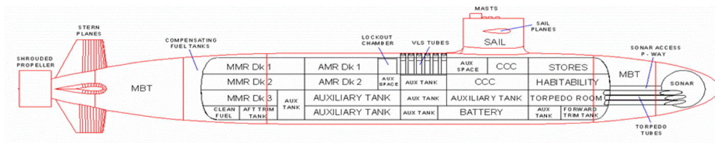
Figure 74 - Profile View Showing Arrangements
