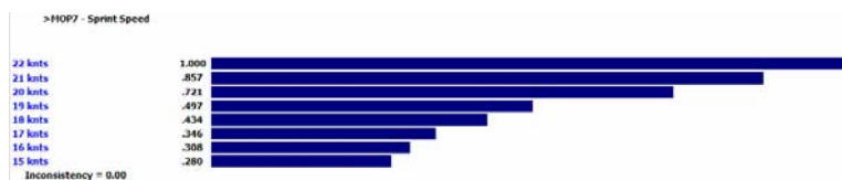
Figure 31 - Value of performance weights for sprint speed
