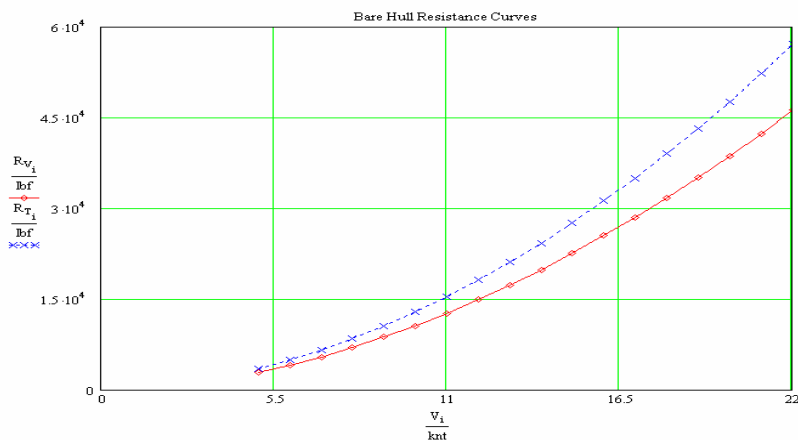
Figure 61 - Submerged Bare Hull Resistance versus Speed
