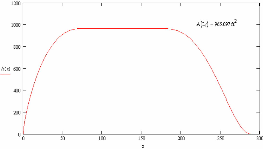
Figure 120 - MathCAD Hullform Module (cont.)
