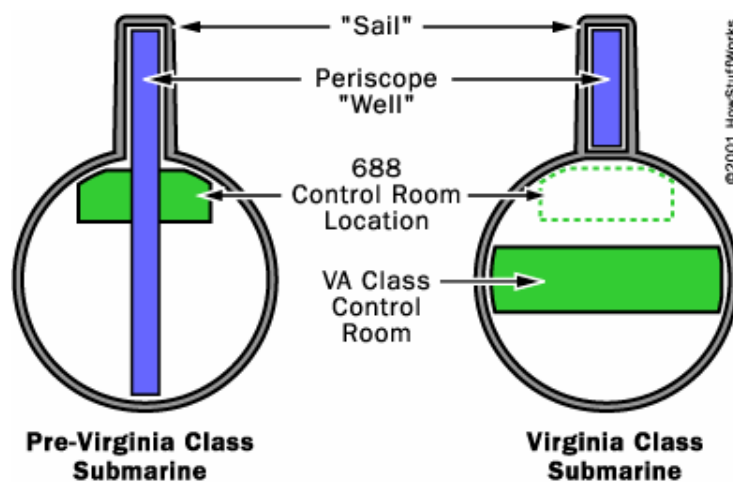
Figure 14 - Traditional and non-hull-penetrating masts [HowStuffWorks.com]
