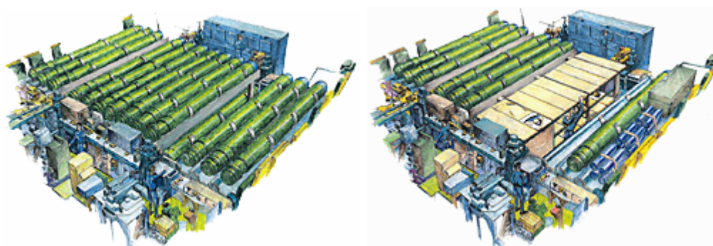
Figure 19 - Torpedo room in two configurations [Dr. Brown, Ship Design Notes]
