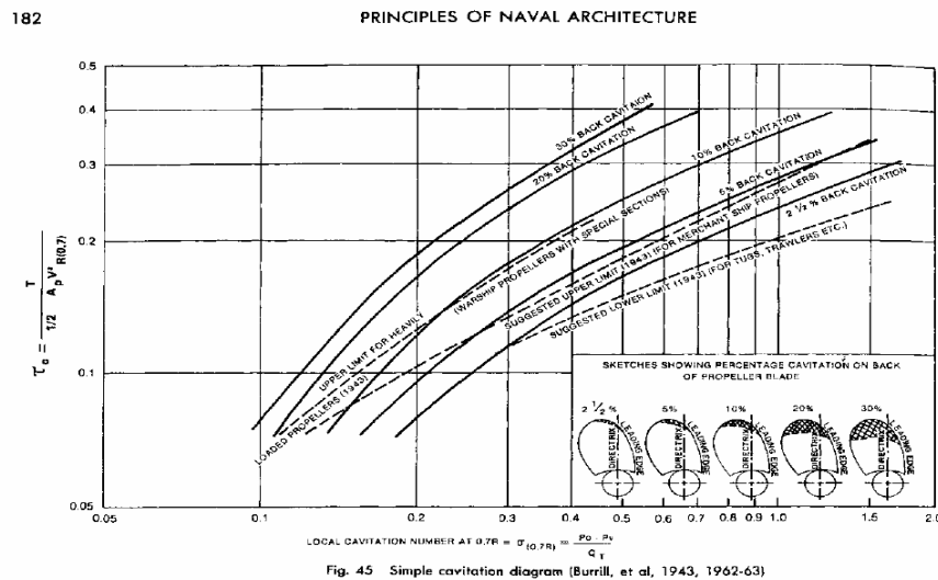
Figure 65 - Burrill's Simple Cavitation Diagram [Principles of Naval Architecture]
