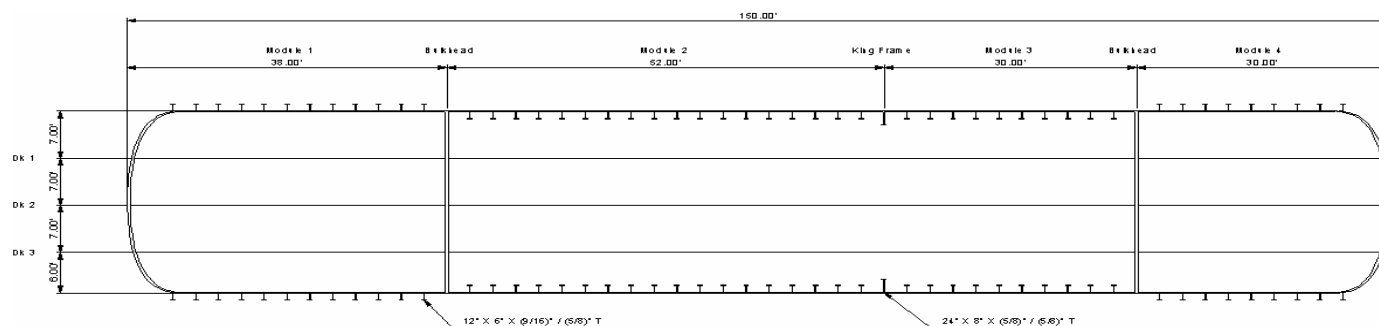
Figure 57 - Longitudinal Structural Profile
