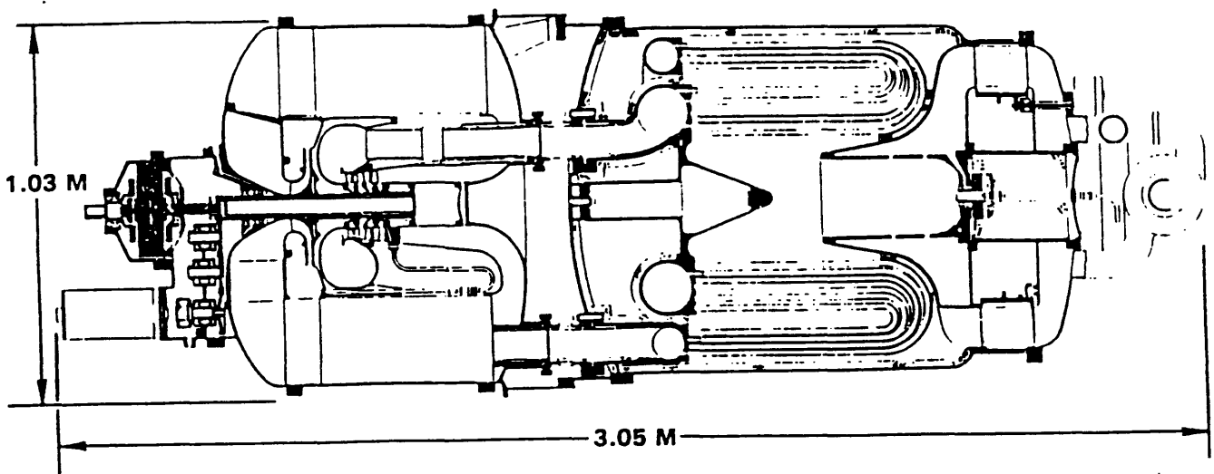
Closed Brayton Cycle Combustion Power System [58]
